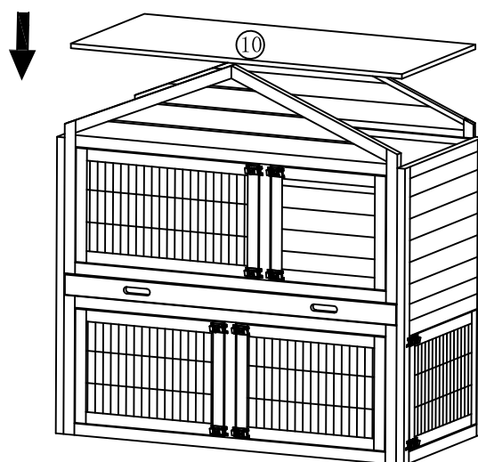
6. Insert the top shelf.
