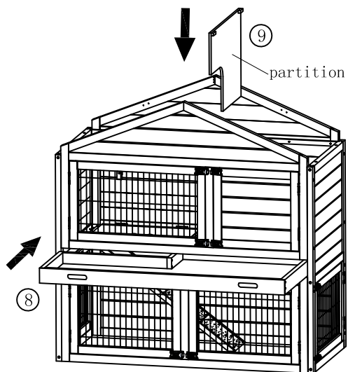
5. Insert the tray and partition.
