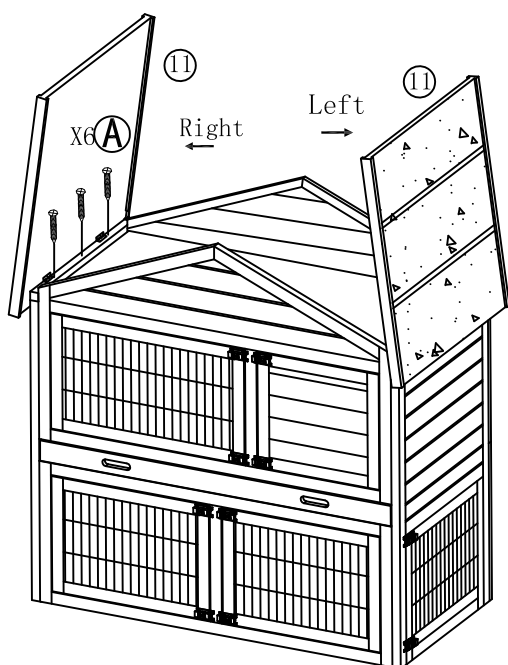
7. Fix the roofs.
